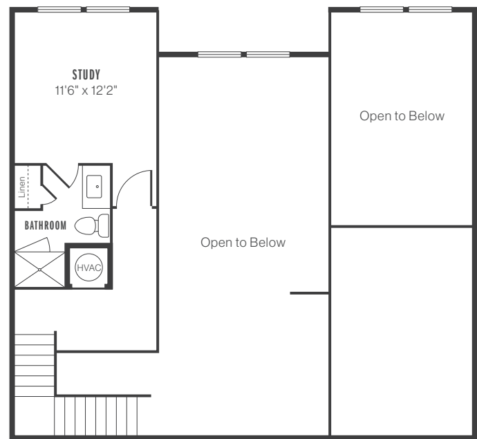
Upper Level
